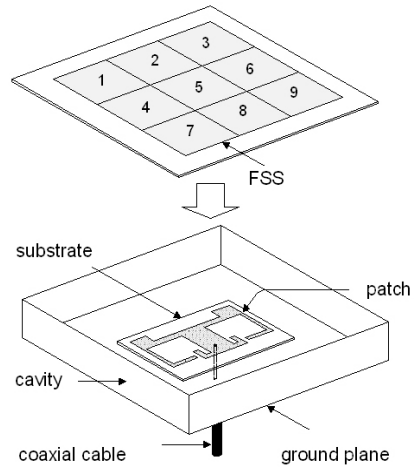
(b) 입체도 (b) Side view
